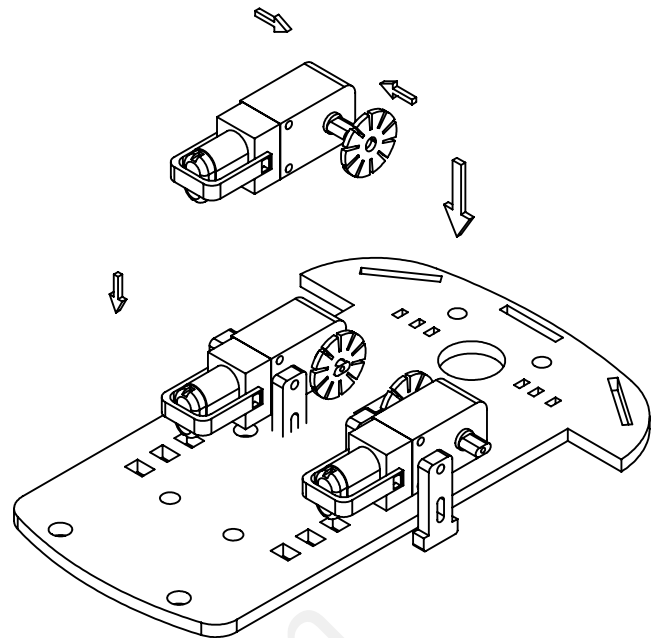
Setp2:assembly the motors as below
