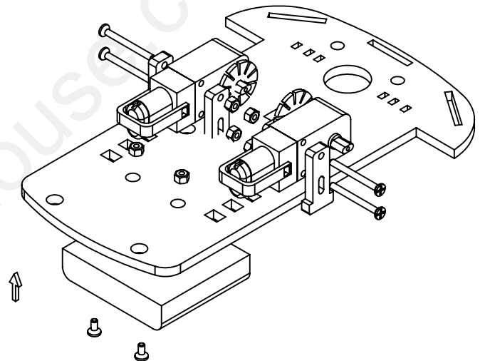
Setp4:assembly the motors as below and assembly battery holder
