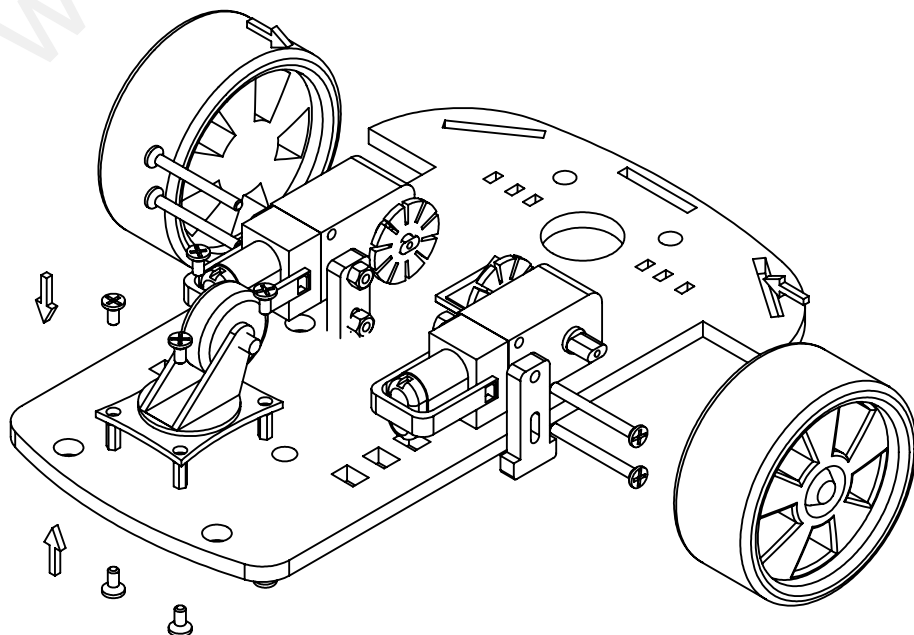
Setp5:assembly omni wheel and assembly wheel
